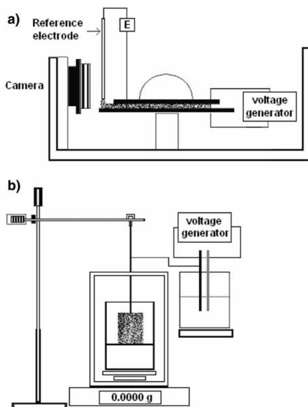
Fig. 1 Schemes of experimental devices for a wetting and b capillary rise measurements under the influence of potential
