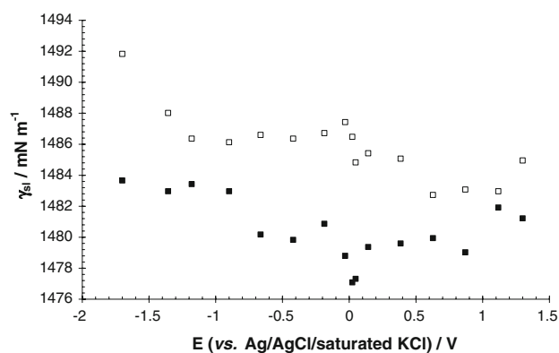
Fig. 3 Electrocapillary curve for the 12.8 \times 10^{-3} M KHT aqueous solution–316L stainless steel interface. The empty squares represent the solution–smooth surface interface. The filled squares represent the solution–rough surface interface
